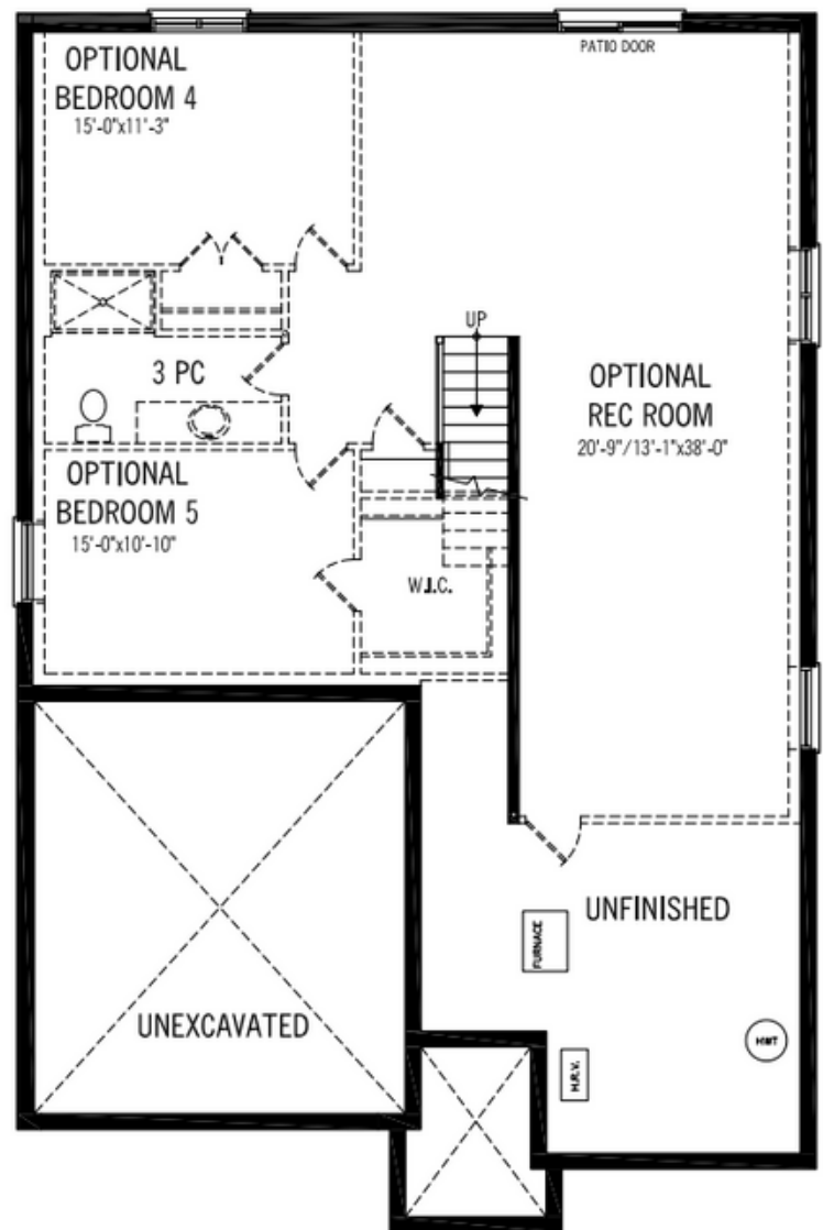
BASEMENT PLAN OPTIONAL FINISHED AREA - 1362 SQ.FT.
