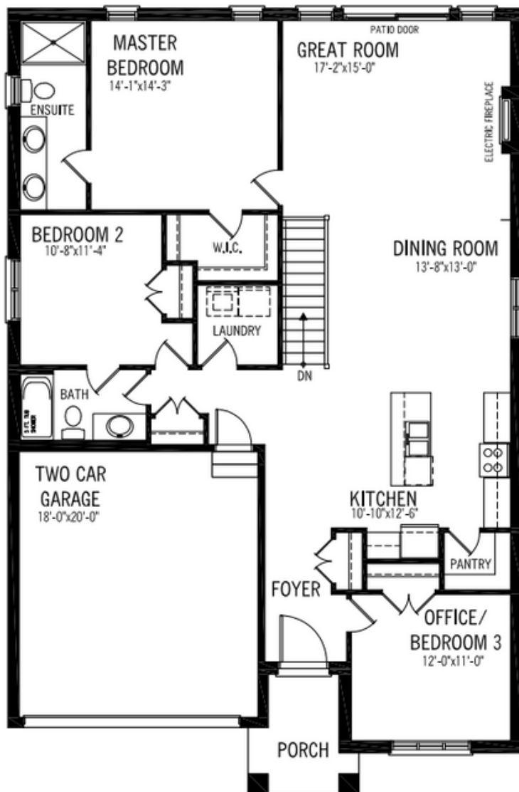
MAIN FLOOR PLAN 1707 SQ.FT.
