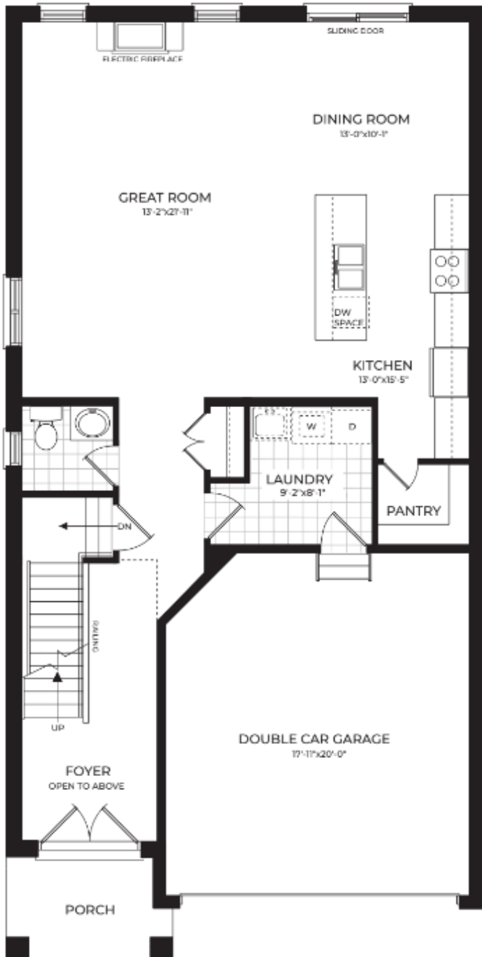
MAIN FLOOR PLAN - 1068 SQ. FT.
