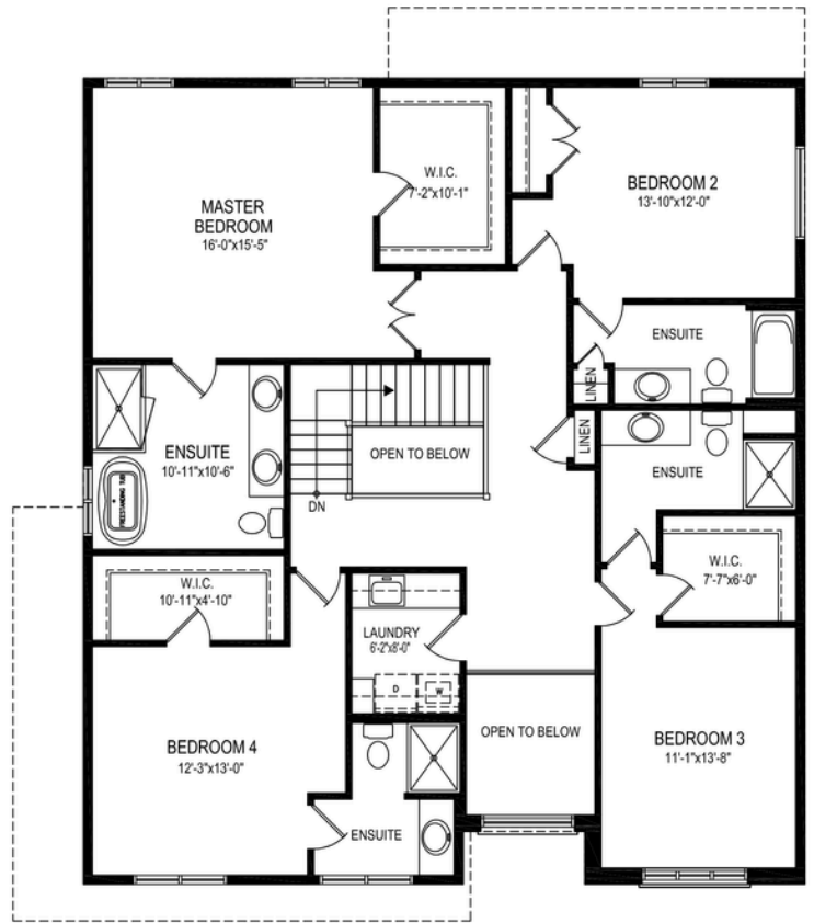
SECOND FLOOR PLAN - 1768 SQ.FT. PLUS 87 SQ.FT. SPACE OPEN TO BELOW
